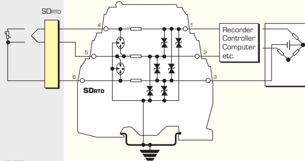
3 wire RTDs
