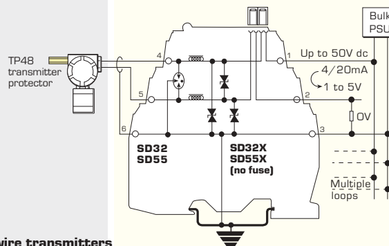
2-wire transmitters
